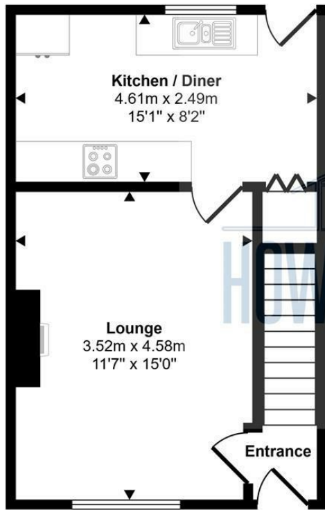
Ground Floor Approx 33 sq m / 353 sq ft
